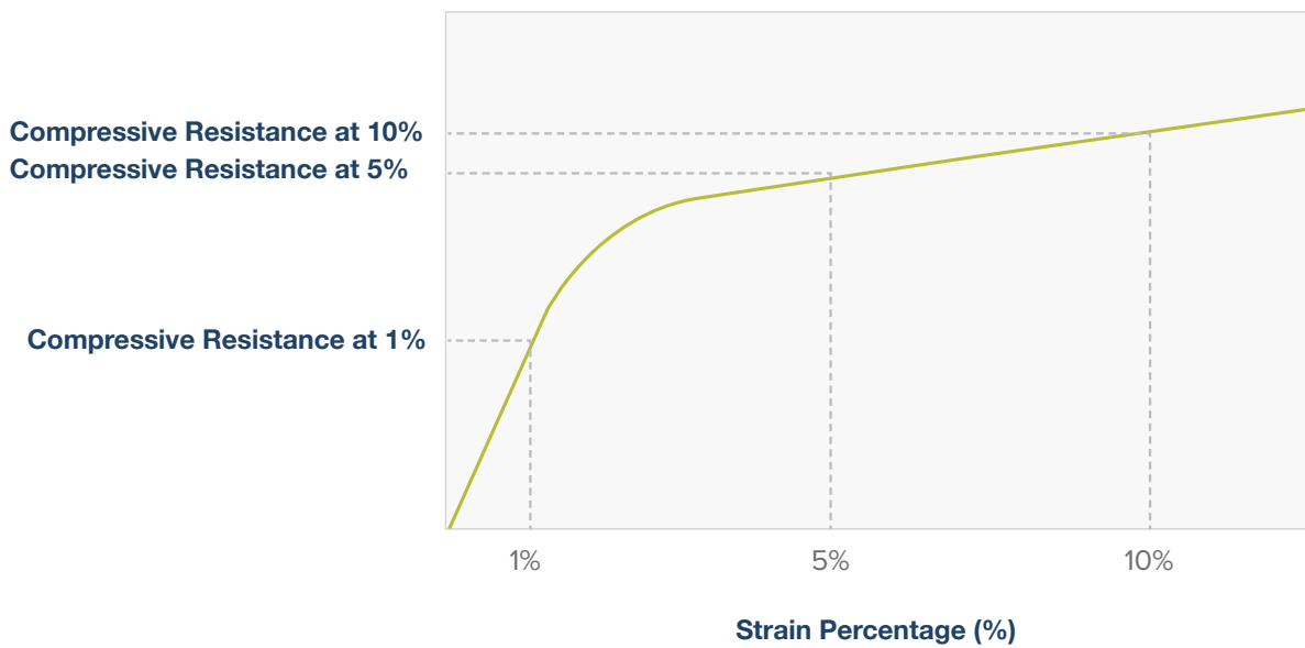
Stress-strain relationship for GeoFoam
